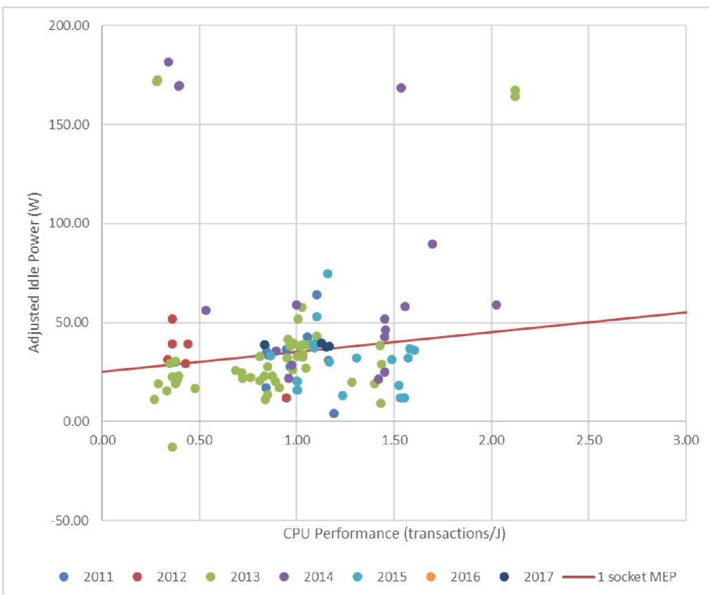
Figure 3 1 socket server idle power adjusted for memory, storage and network adders vs. proposed idle requirement
