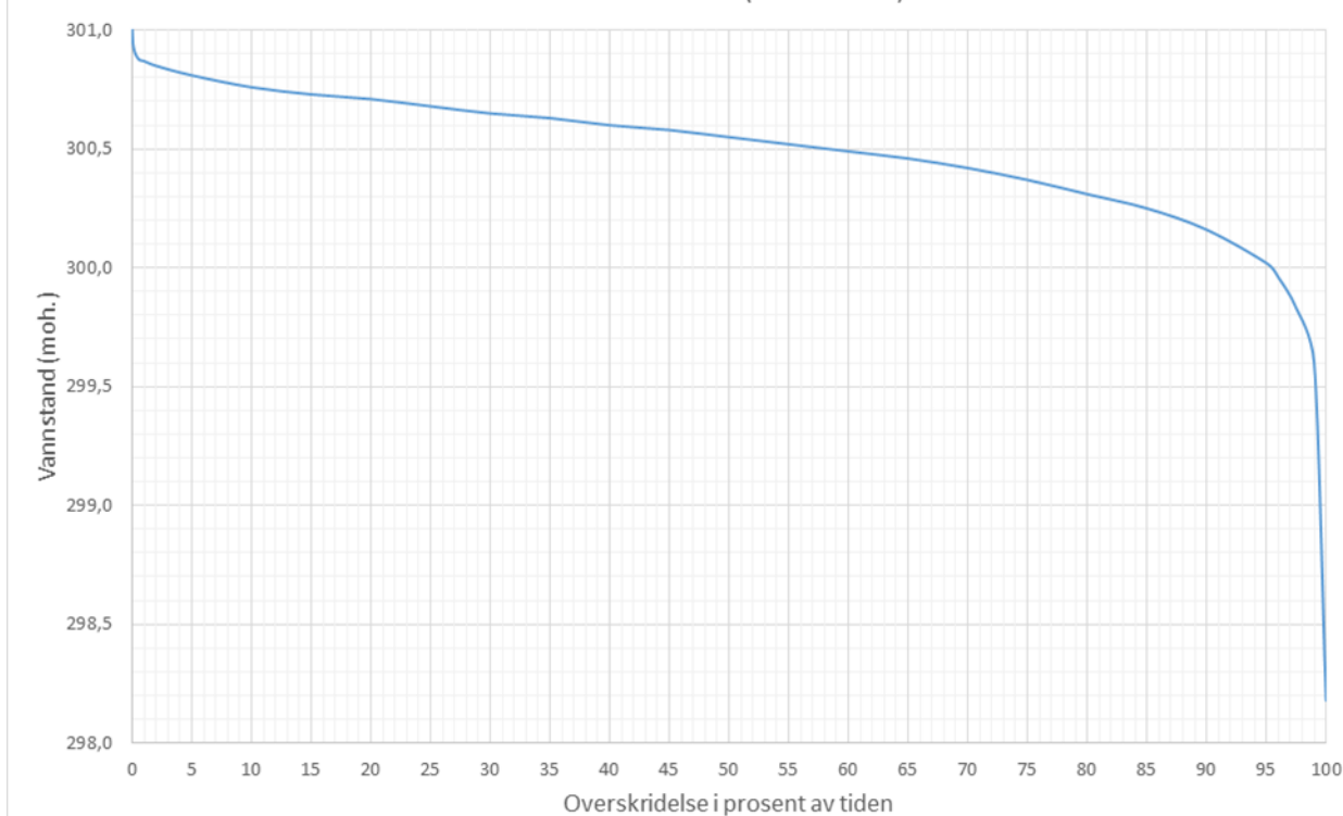
Vannstand i Innsetvatn (2007 - 2017)
