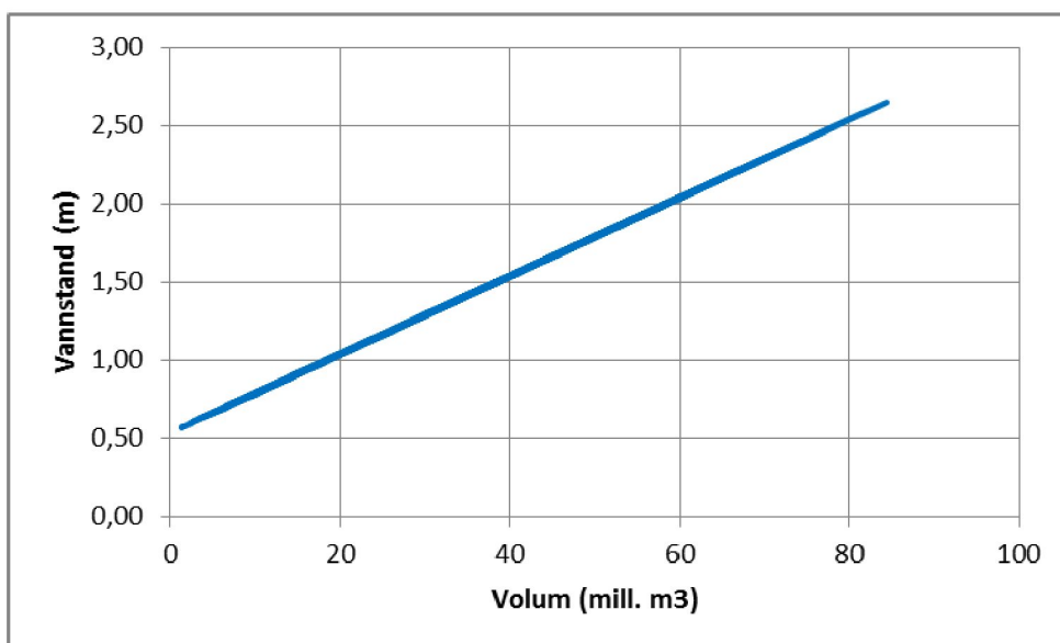
Figur 4. Magasinkurve for Jølstravatnet.
