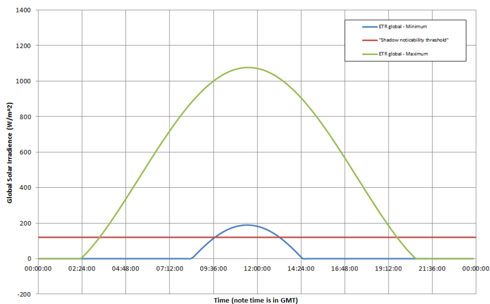
Maximum and Minimum Solar Radiation (20th June 2014 and 21st December 2014)
