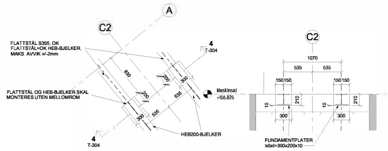
Detalj 3 Bjelker 1 : 25
