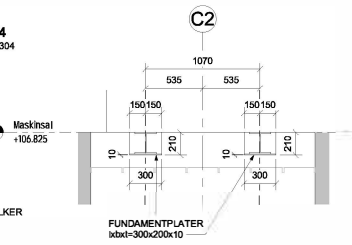
Detalj 4 Bjelker 1 : 25
