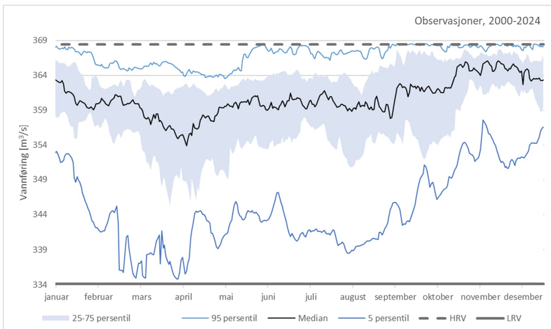
Figur 5-2 Persentilkurver for observerte data for perioden 2000-2024
