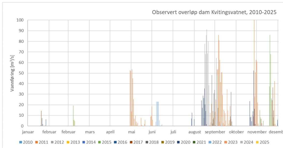
Figur 5-8 Historiske overløpsepisoder, dam Kvittingsvatnet
