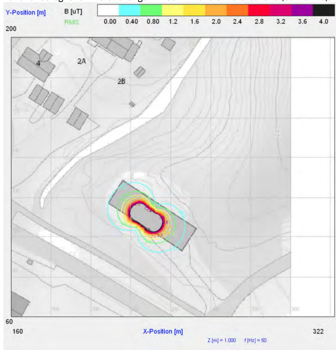
Figur 41: Magnetfeltberegning
