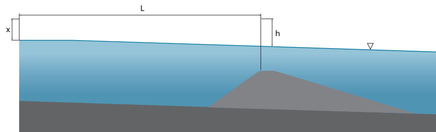
Figur 8.28 Terskeloppstuving.
