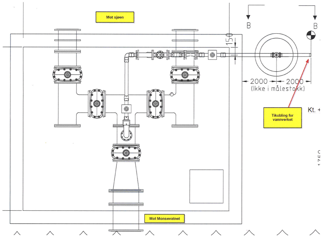
Plan kum
