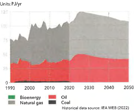
FIGURE 2.12 Norway non-energy demand for energy carriers
