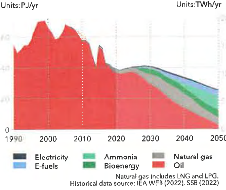
Norway maritime subsector energy demand by carrier
