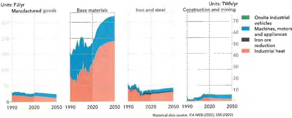
FIGURE 2.10 Norway manufacturing subsectors energy demand by end use
