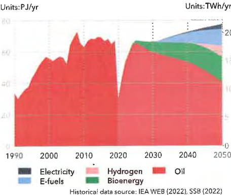
Norway aviation subsector energy demand by carrier
