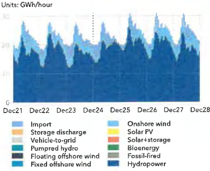
Norway electricity supply by source; week 52; 2026
